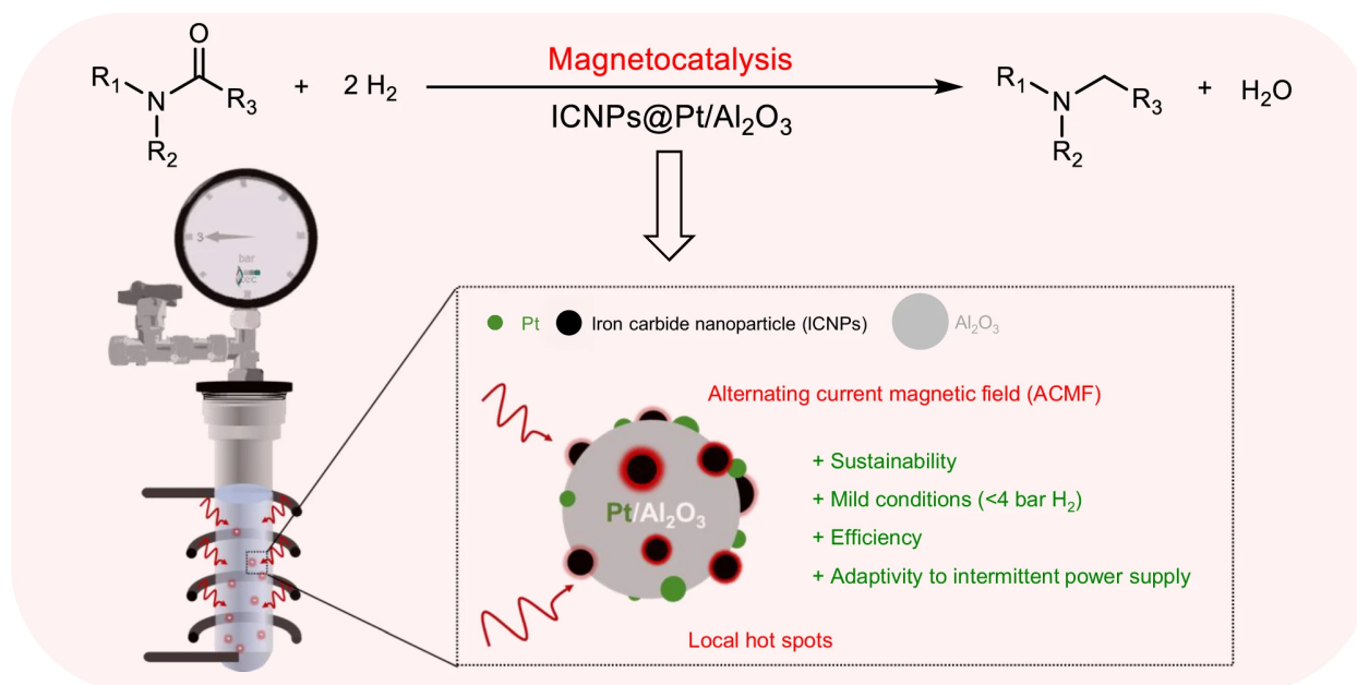
Figure 1: Magnetocatalytic amide hydrogenation using \text{ICNPs@Pt}/\text{Al}_2\text{O}_3 under ACMF enables efficient, low-pressure conversion to amines with localized heating and high selectivity.
